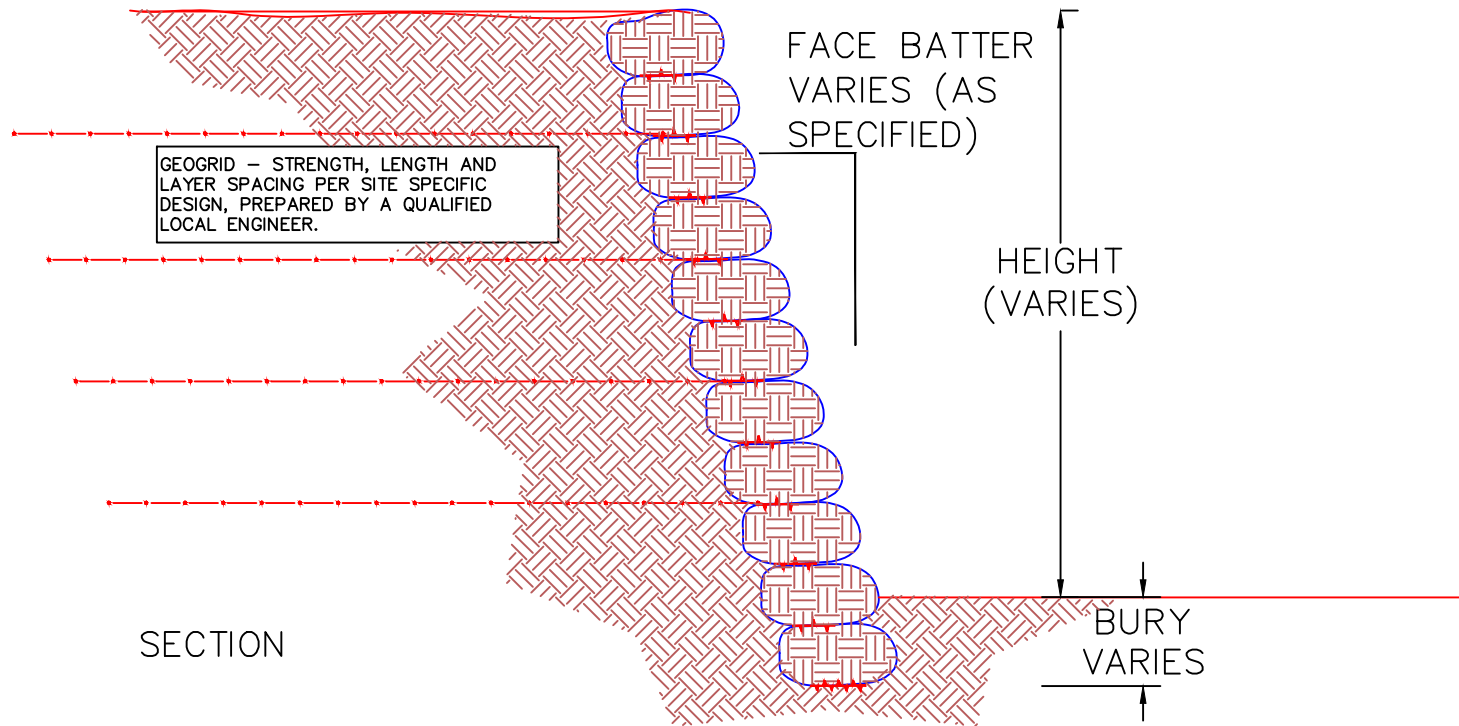
3 GEOGRID REINFORCED FLEX MSE WALL; TYPICAL
