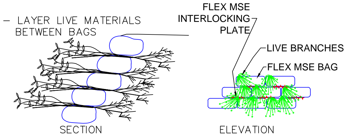
3 VEGETATION - BRUSH LAYERING
